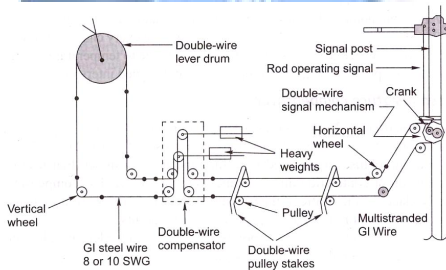
Fig: b Double wire Transmission system
