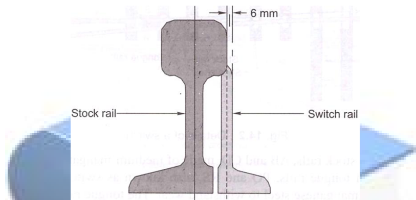
Fig. Undercut switch
