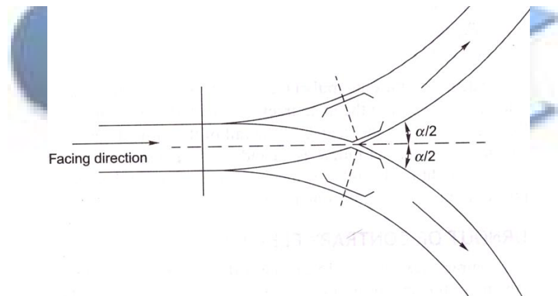
Fig. Symmetrical split
