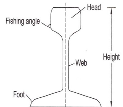
FLAT-FOOTED RAIL
