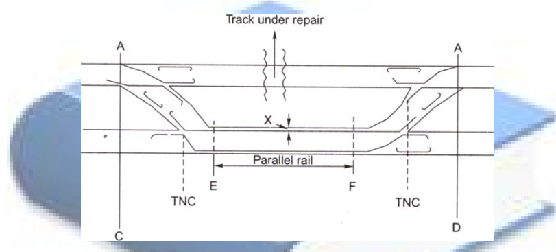
Fig. (a) Gauntletted track
